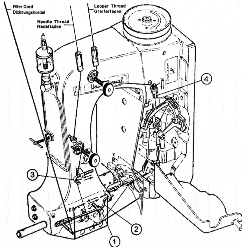
Needle Thread Threading on styles 80800CN, HN and HAN
